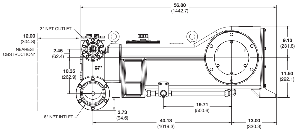
Side View
