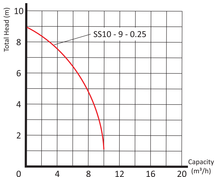
Performance curve
