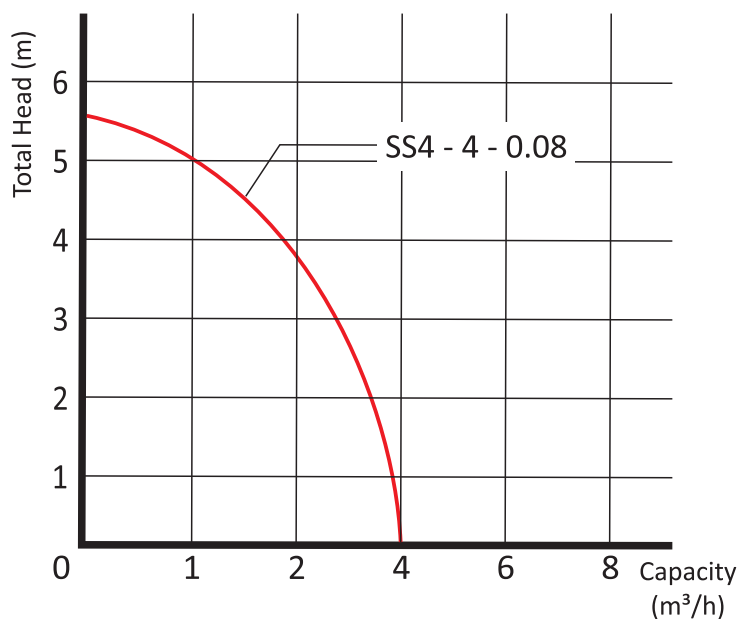
Performance curve
