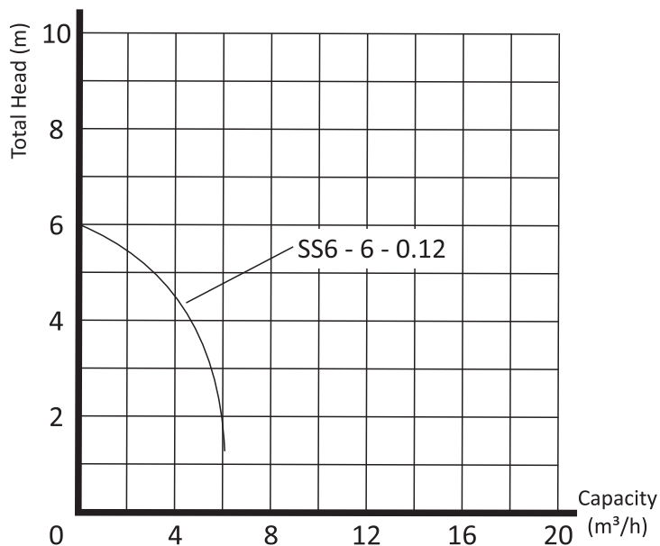
Performance curve
