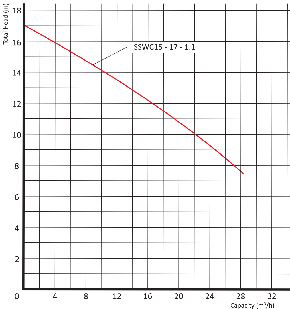
Performance curve
