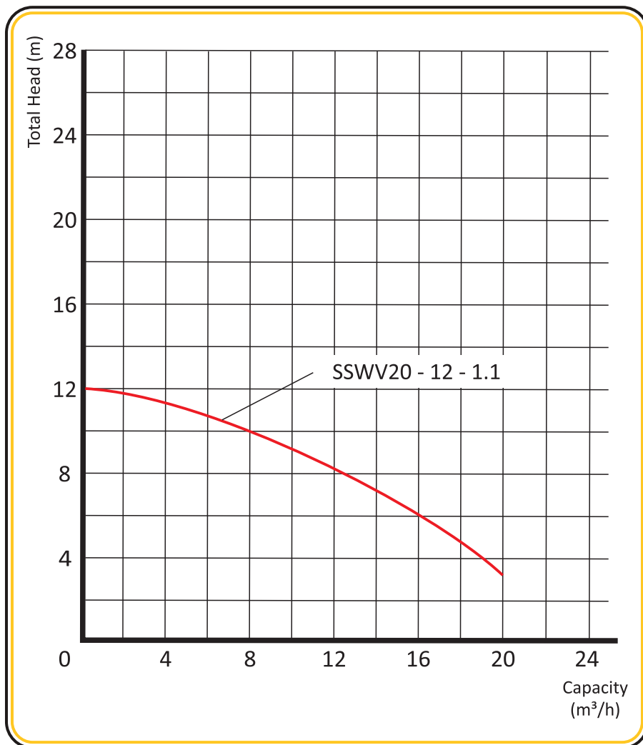
Performance curve
