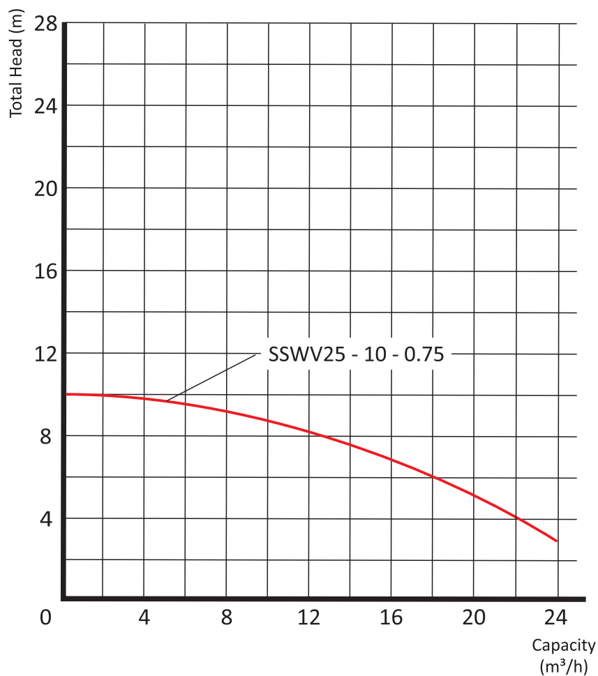
Performance curve
